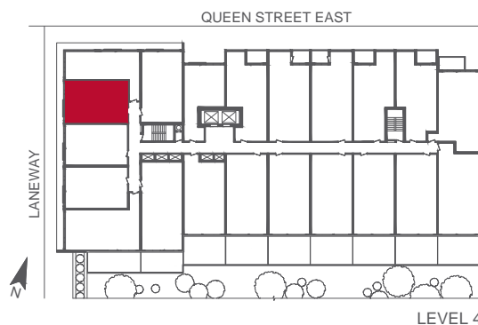
LEVEL 4
